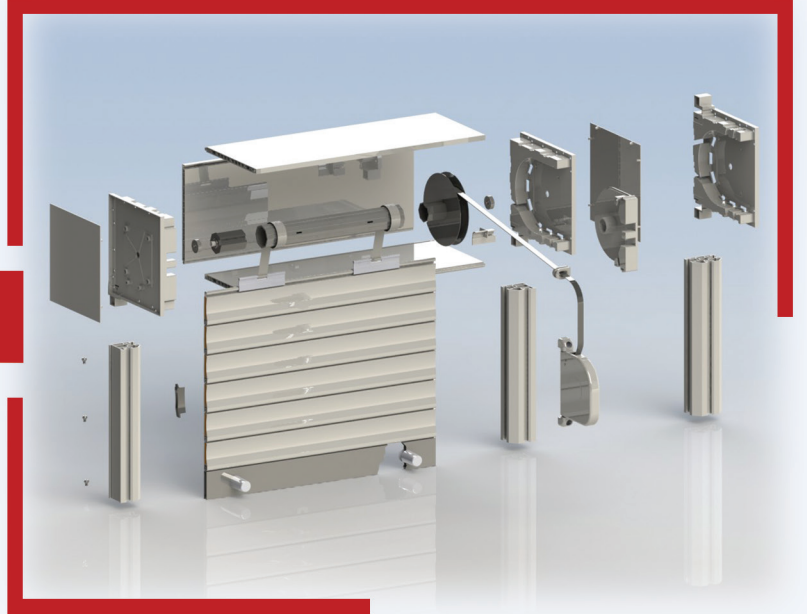
MONOBLOK PANJUR SİSTEMİ MONOBLOCK ROLLING SHUTTER SYSTEM
