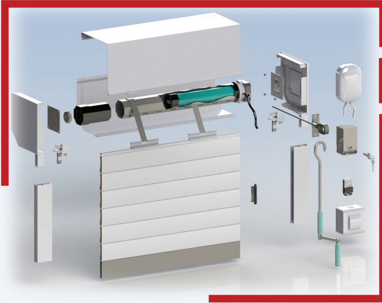
ALÜMİNYUM MOTORLU PANJUR VE KEPENK SİSTEMİ ALUMINIUM MOTORIZED SHUTTER SYSTEM
