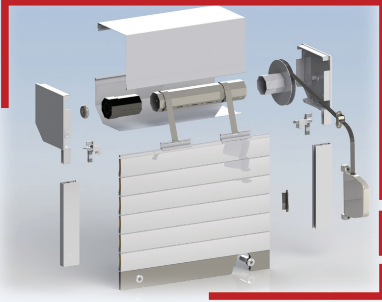
ALÜMİNYUM MAKARALI PANJUR SİSTEMİ ALUMINIUM MANUAL SHUTTER SYSTEM
